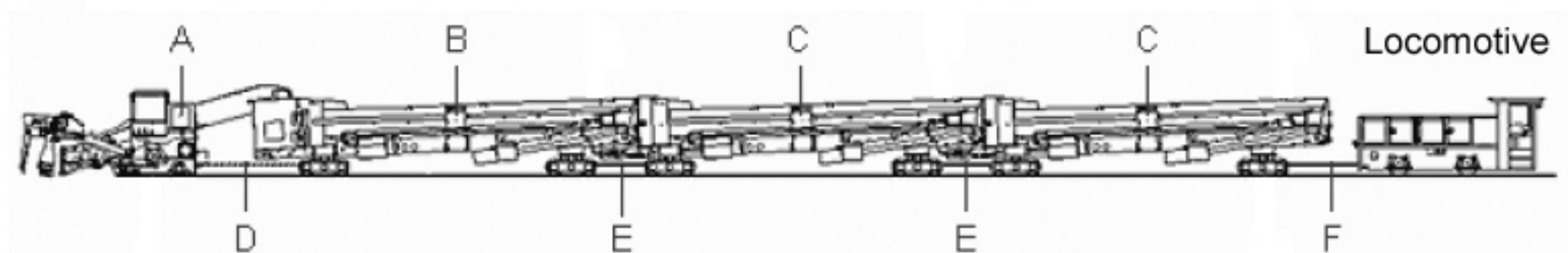
HAGGLOADER AND SHUTTLE CARS
